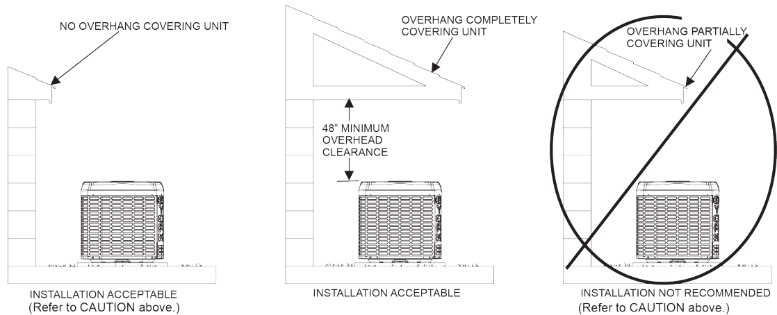
Figure 3: Overhang positioning
