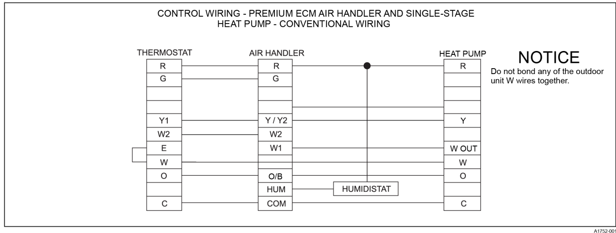
Figure 9: Standard SS HP - Premium ECM Gas Furnace
